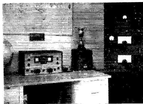
The top Canadian score, 100,013 points, was tallied from this neat operating position by Cliff Tallier, VE5QZ.
