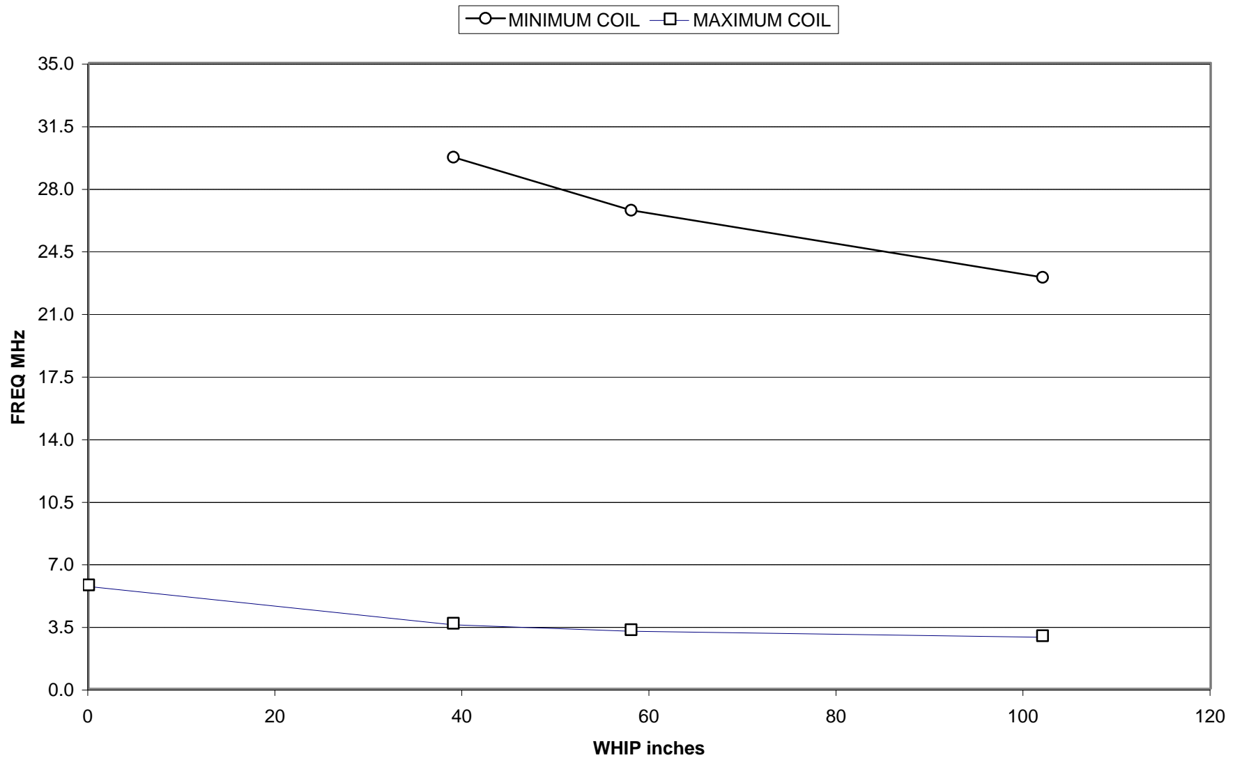
Frequency versus Whip Length
